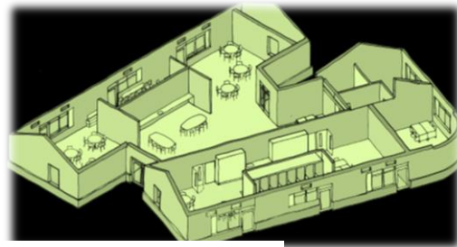
Early Years Pavilion Plan
